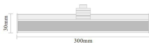
Transducer
